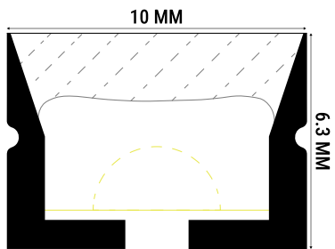
LED STRIP STRUCTURE
