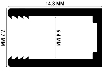
ALUMINUM RAIL
