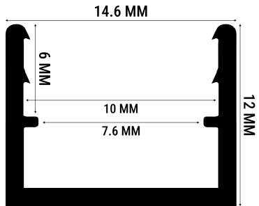
PVC RAIL
