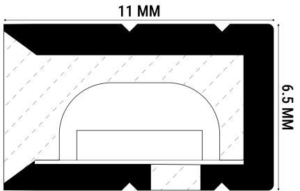
LED STRIP STRUCTURE
